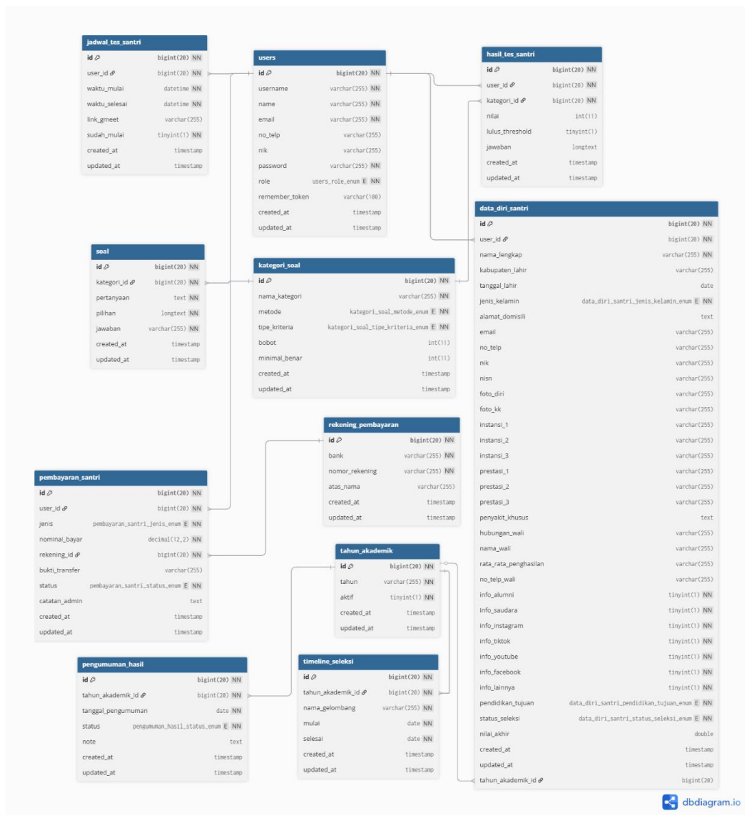
Gambar 3.7 Class Diagram
